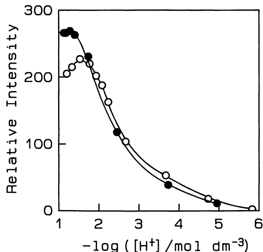
Fig. 2. Relative fluorescent intensity as a function of the concentration of acid used for postcolumn hydrolysis of 5 . Column, 150×6 mm i.d. Shim-pack CLC-ODS; eluent, methanol 1.0 ml \text{min}^{-1} ; post-column reagent, (●) nitric acid or (○) hydrochloric acid at 0.2 ml \text{min}^{-1} ; sample size, 10 \mu\text{l} (66 pmol); detector, Shimadzu RF-5000, \lambda_{\text{ex}}=334 nm, \lambda_{\text{em}}=398 nm (slit widths 15 nm).
